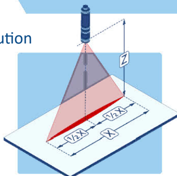
(b) Vertical installation (perpendicular 90°)
